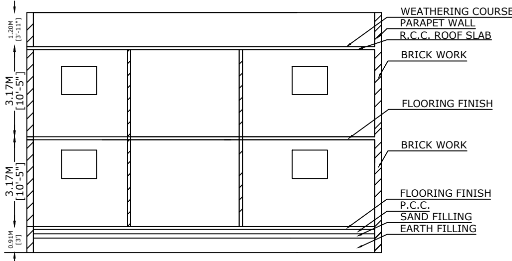
SECTION AN AA
