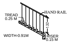
STAIRCASE DETAILS
