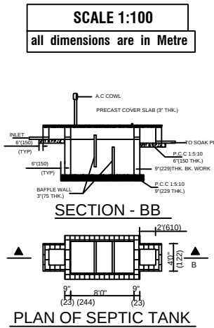
PLAN OF SEPTIC TANK
