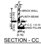
SECTION - CC
