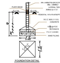
FOUNDATION DETAIL
