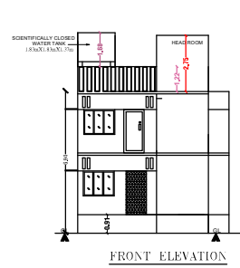
FRONT ELEVATION
