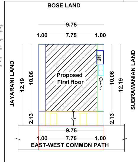
SITE PLAN & KEY PLAN (1:100)
