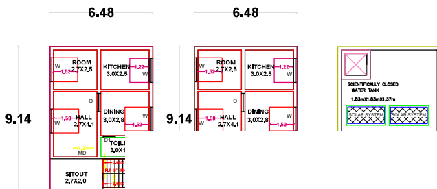
GROUND FLOOR
