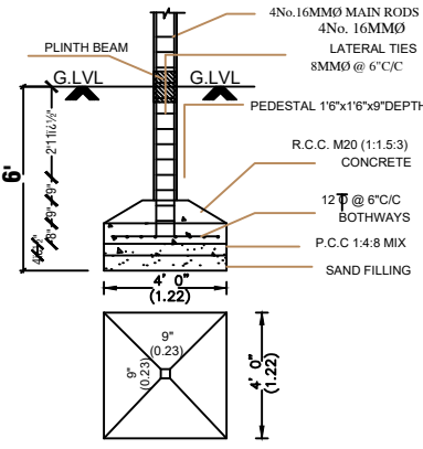
FOUNDATION DETAIL
