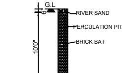
PERCOLATION PIT
