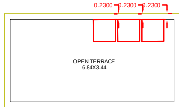
TERRACE FLOOR PLAN PROPOSED
