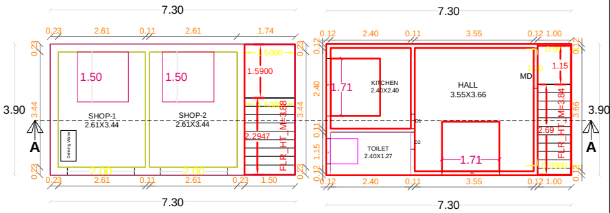
GROUND FLOOR PLAN PROPOSED
