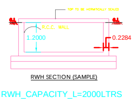
RWH_CAPACITY_L=2000LTRS
