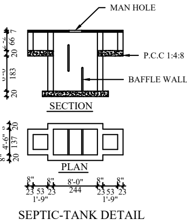
SEPTIC-TANK DETAIL
