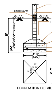
FOUNDATION DETAIL
