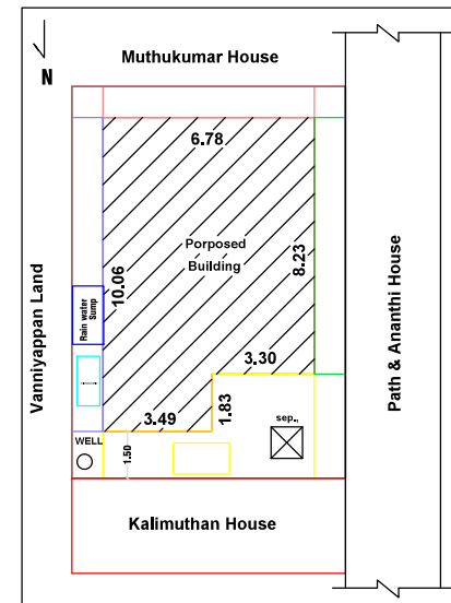
SITE PLAN CUM KEYPLAN
