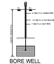
BORE WELL
