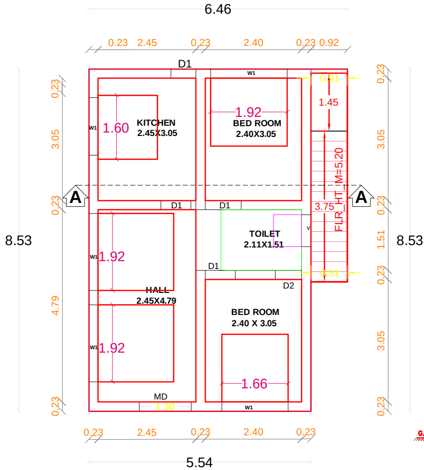
GROUND FLOOR PLAN PROPOSED
