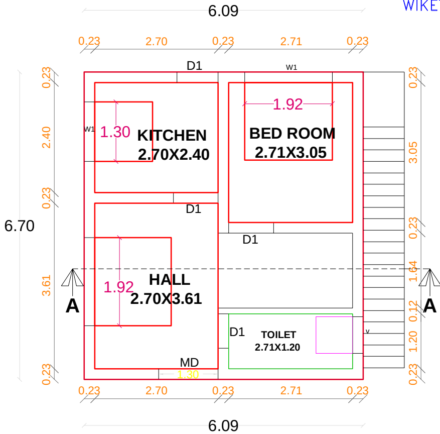
GROUND FLOOR PLAN PROPOSED
