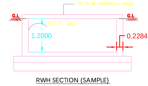
RWH_CAPACITY_L=2000LTRS
