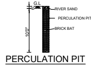
PERCOLATION PIT
