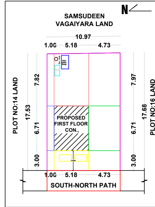
SITE PLAN & KEY PLAN (1:100)
