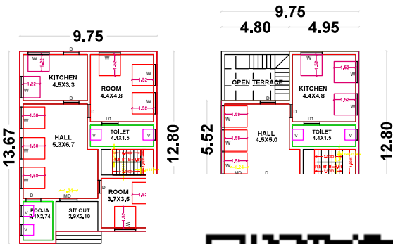
GROUND FLOOR I
