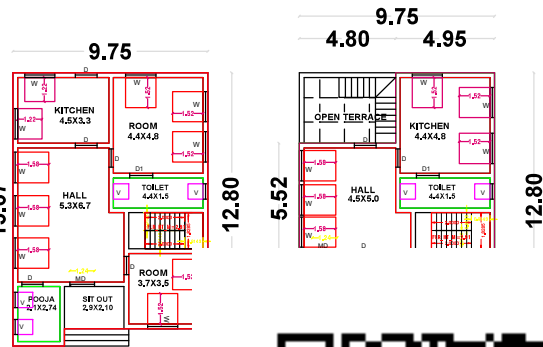
GROUND FLOOR P
