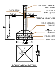
FOUNDATION DETAIL
