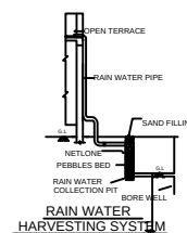
RAIN WATER HARVESTING SYSTEM
