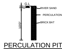
PERCOLATION PIT
