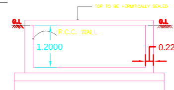
RWH SECTION (SAMPLE) RWH_CAPACITY_L=2000LTRS
