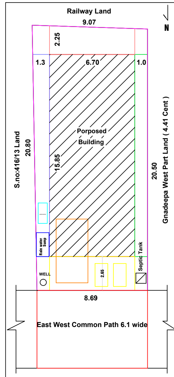
SITE PLAN CUM KEYPLAN
