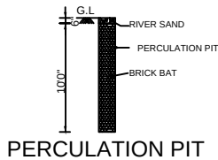
PERCOLATION PIT
