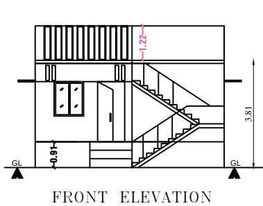
FRONT ELEVATION
