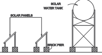
SECTION OF SOLAR HEATER
