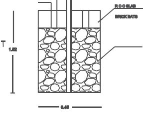
RAIN WATER STORAGE
