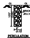
PERCOLATION PIT
