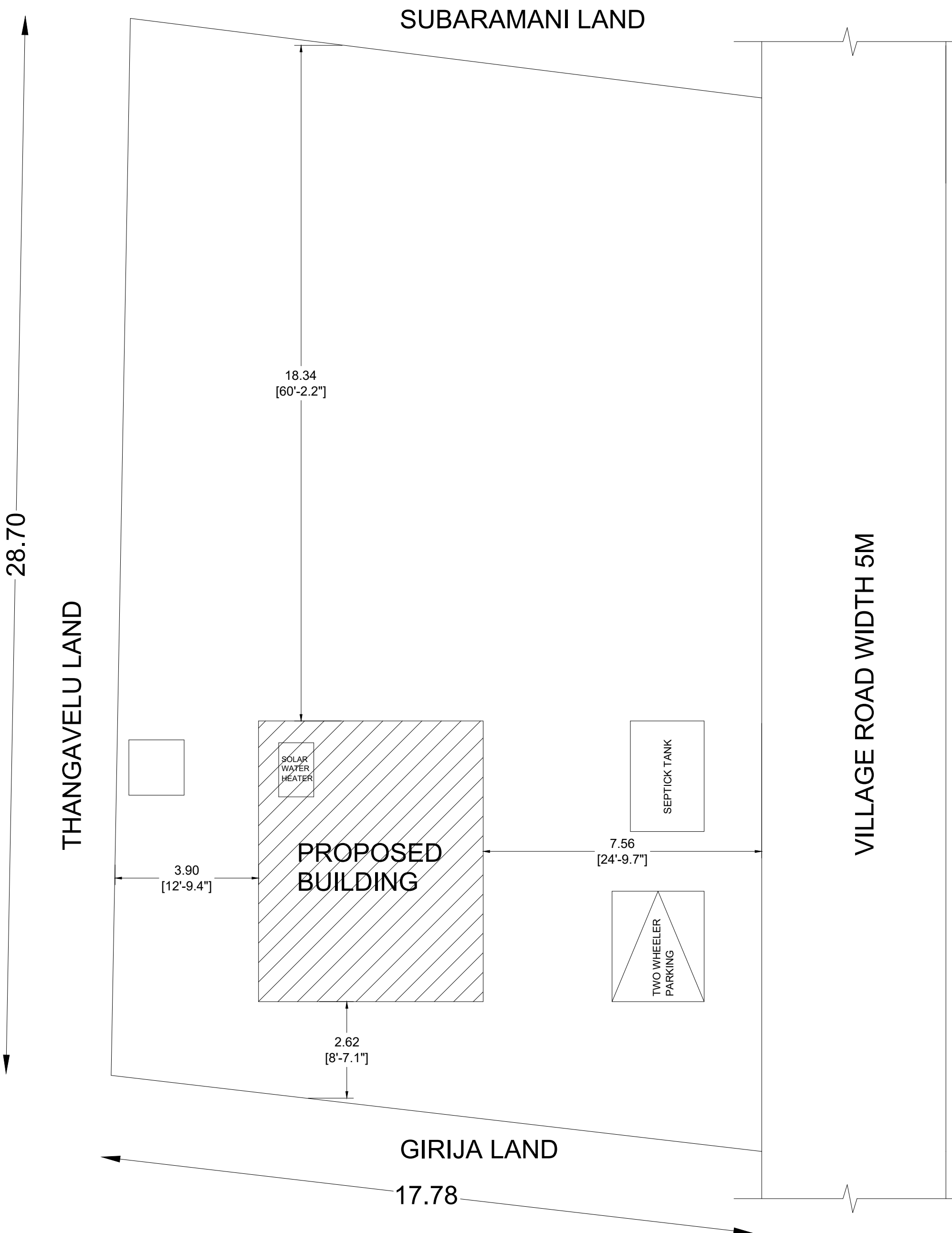
SITE PLAN
