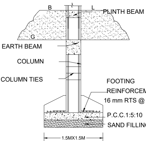
FOUNDATION DETAIL
