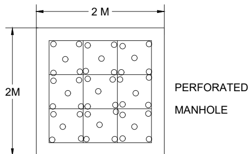
PLAN OF RAIN WATER RECHARGING PIT
