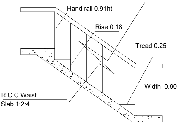
STAIRCASE DETAIL
