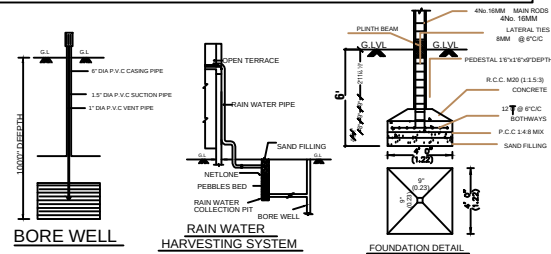
FOUNDATION DETAIL
