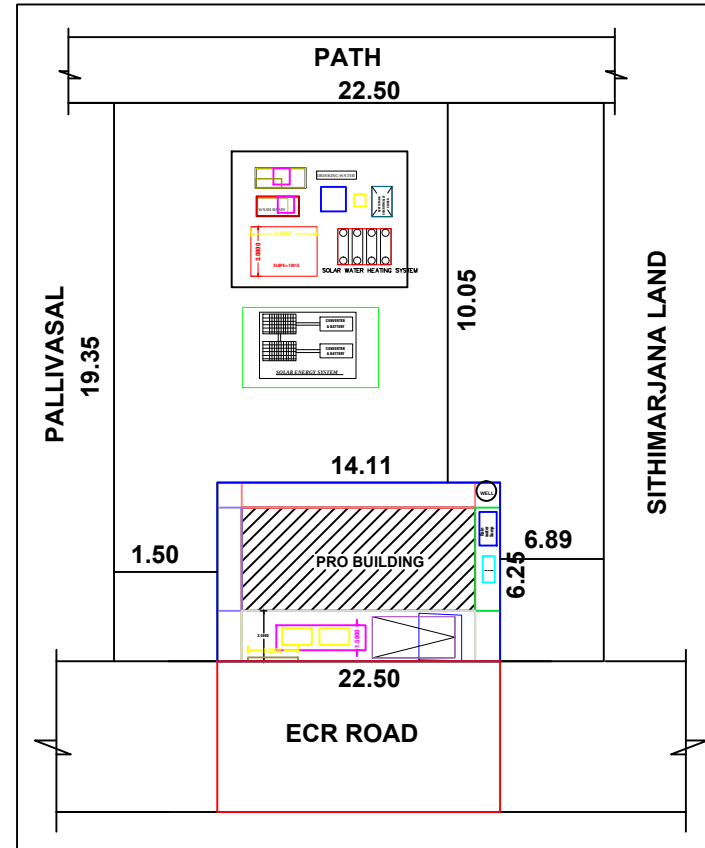
SITE PLAN & KEY PLAN
