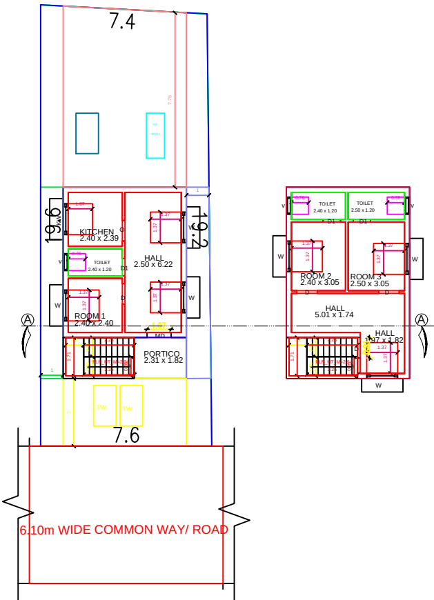
PLAN CUM PROPOSED GROUND FLOOR PLAN
