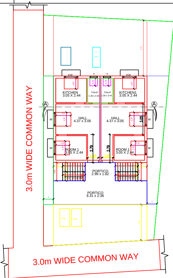
SITE PLAN CUM PROPOSED GROUND FLOOR PLAN
