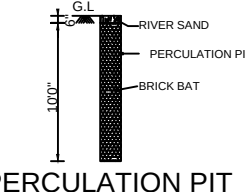
PERCOLATION PIT
