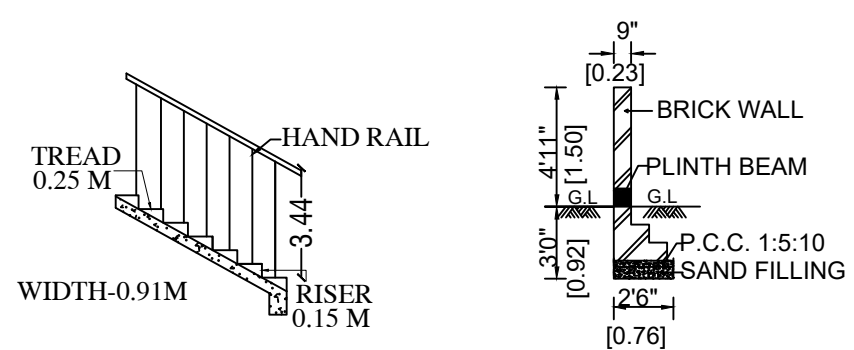
STAIRCASE DETAILS SECTION - CC
