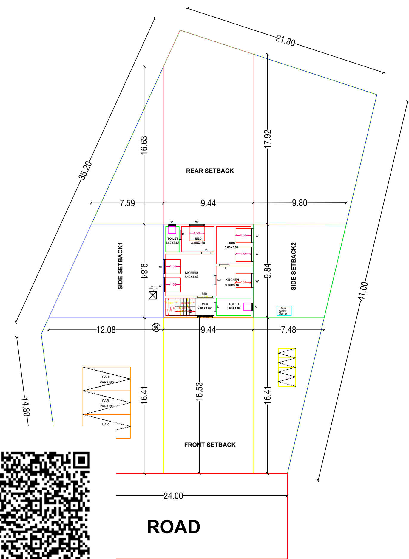
E PLAN CUM GROUND FLOOR PLAN
