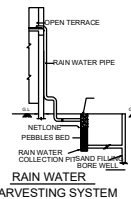
RAIN WATER HARVESTING SYSTEM
