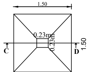
SECTION - 'CD'
