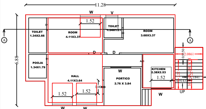
PRO.GROUND FLOOR PLAN
