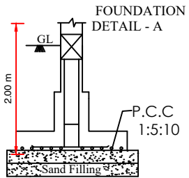
Isolated Footing -A (1.50X1.50) (Not to Scale)
