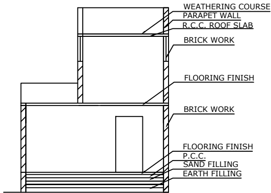
SECTION AN AA
