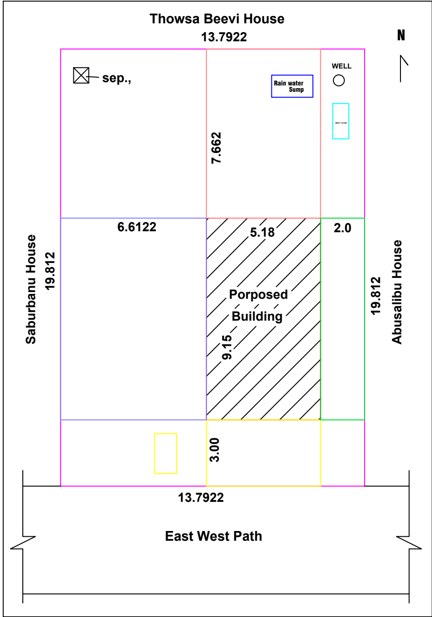
SITE PLAN CUM KEYPLAN
