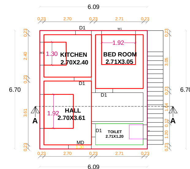
GROUND FLOOR PLAN PROPOSED
