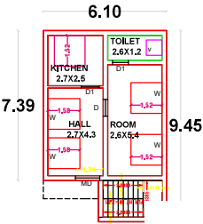
GROUND FLOOR F
