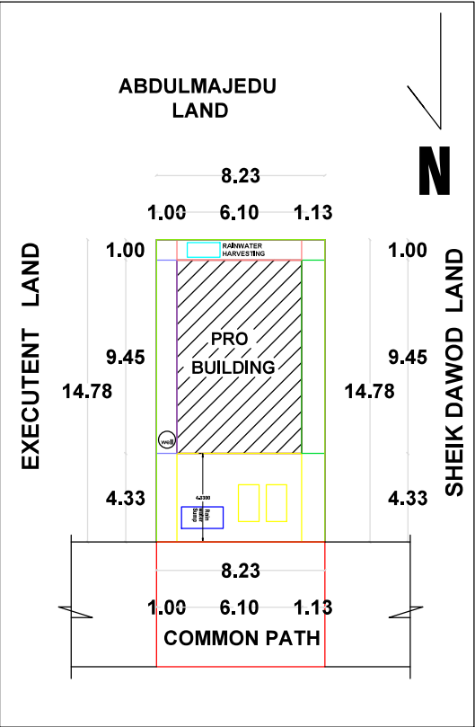
SITE PLAN & KEY PLAN (1:100)
