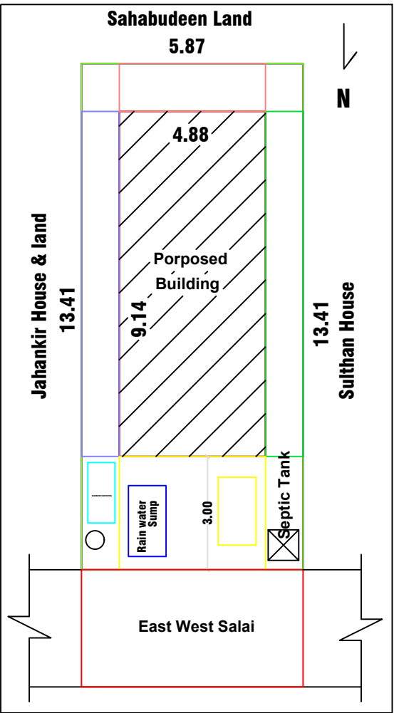
SITE PLAN CUM KEYPLAN
