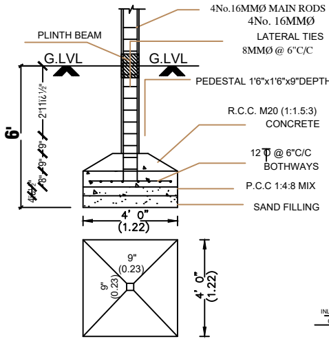
FOUNDATION DETAIL [SCALE: 1:50]
