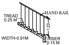
STAIRCASE DETAILS
