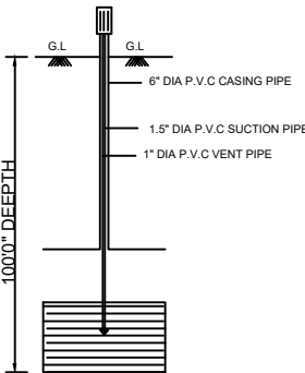
BORE WELL
