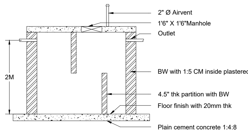
CROSS SECTION OF SEPTIC TANK
