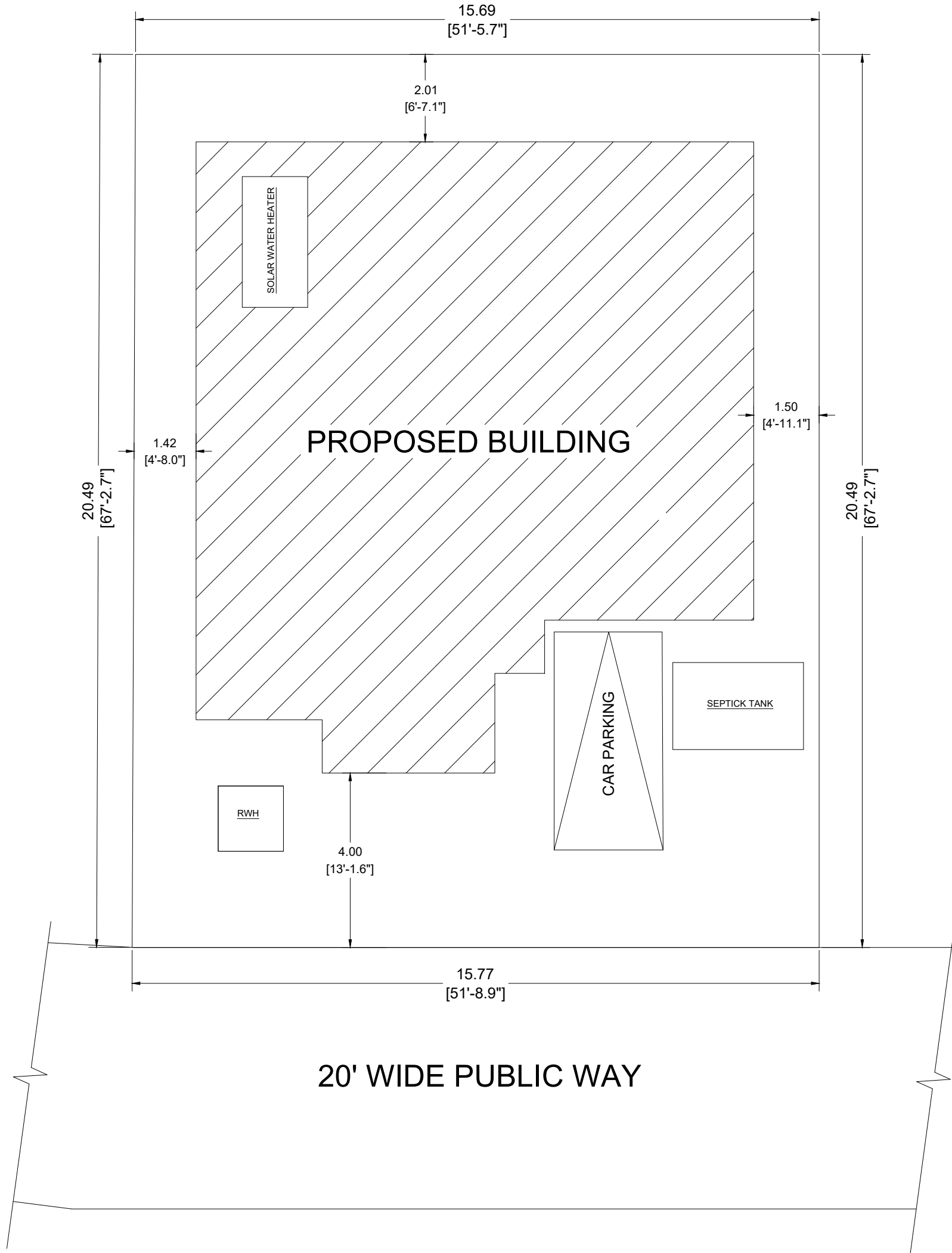
KEY PLAN
