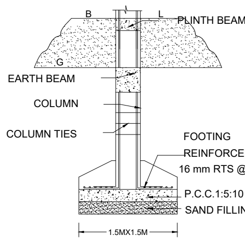
FOUNDATION DETAIL
