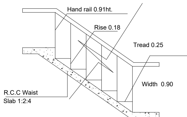
STAIRCASE DETAIL
