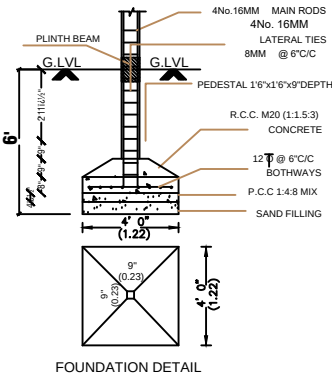
FOUNDATION DETAIL
