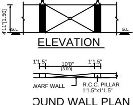
GROUND WALL PLAN
