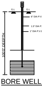
BORE WELL
