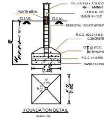
FOUNDATION DETAIL
