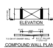
COMPOUND WALL PLAN
