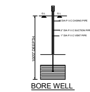
BORE WELL
