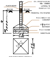
FOUNDATION DETAIL
