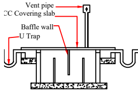
Section Plan
