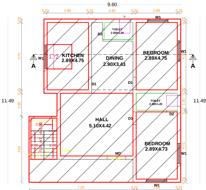
FIRST FLOOR PLAN PROPOSED
