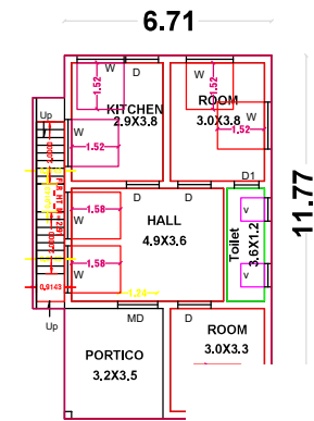
GROUND FL
