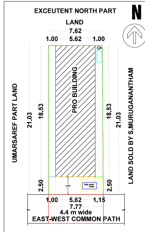
SITE PLAN & KEY PLAN
