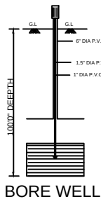
BORE WELL
