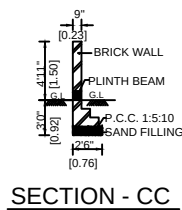
PERCOLATION PIT
