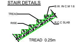
STAIR DETAILS
