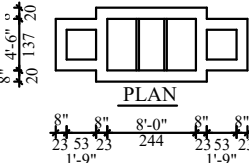
SEPTIC-TANK DETAIL
