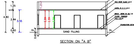
SECTION ON "A B"
