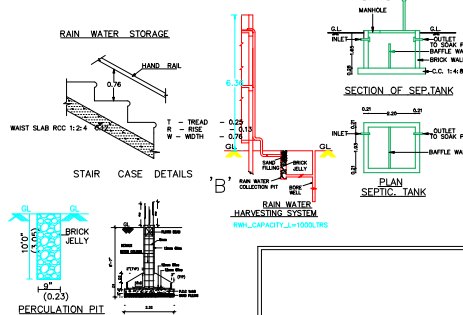
RAIN WATER HARVESTING SYSTEM SCALE : 1:50
