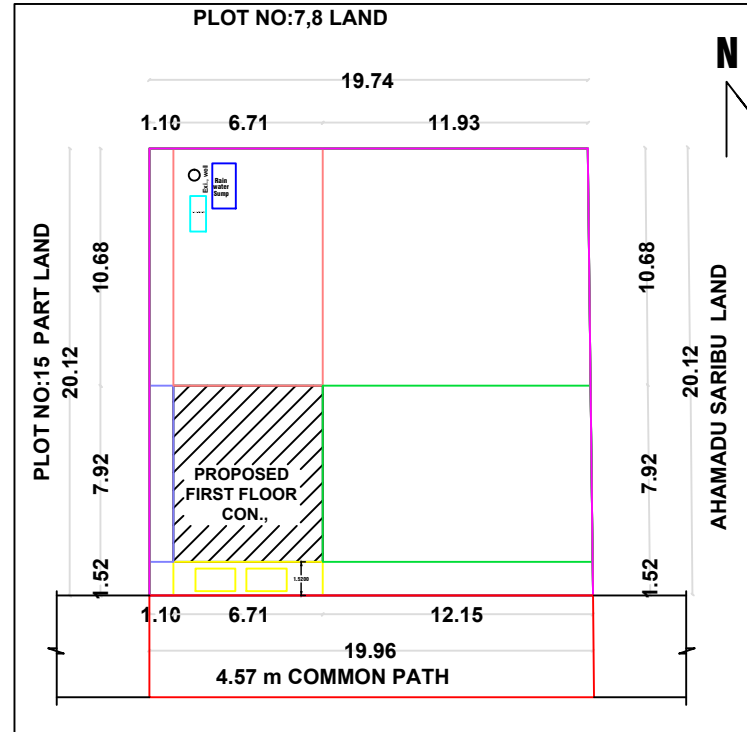
SITE PLAN & KEY PLAN (1:100)
