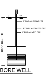
BORE WELL
