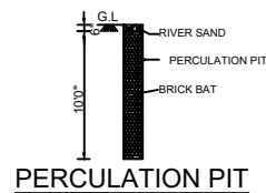
PERCOLATION PIT
