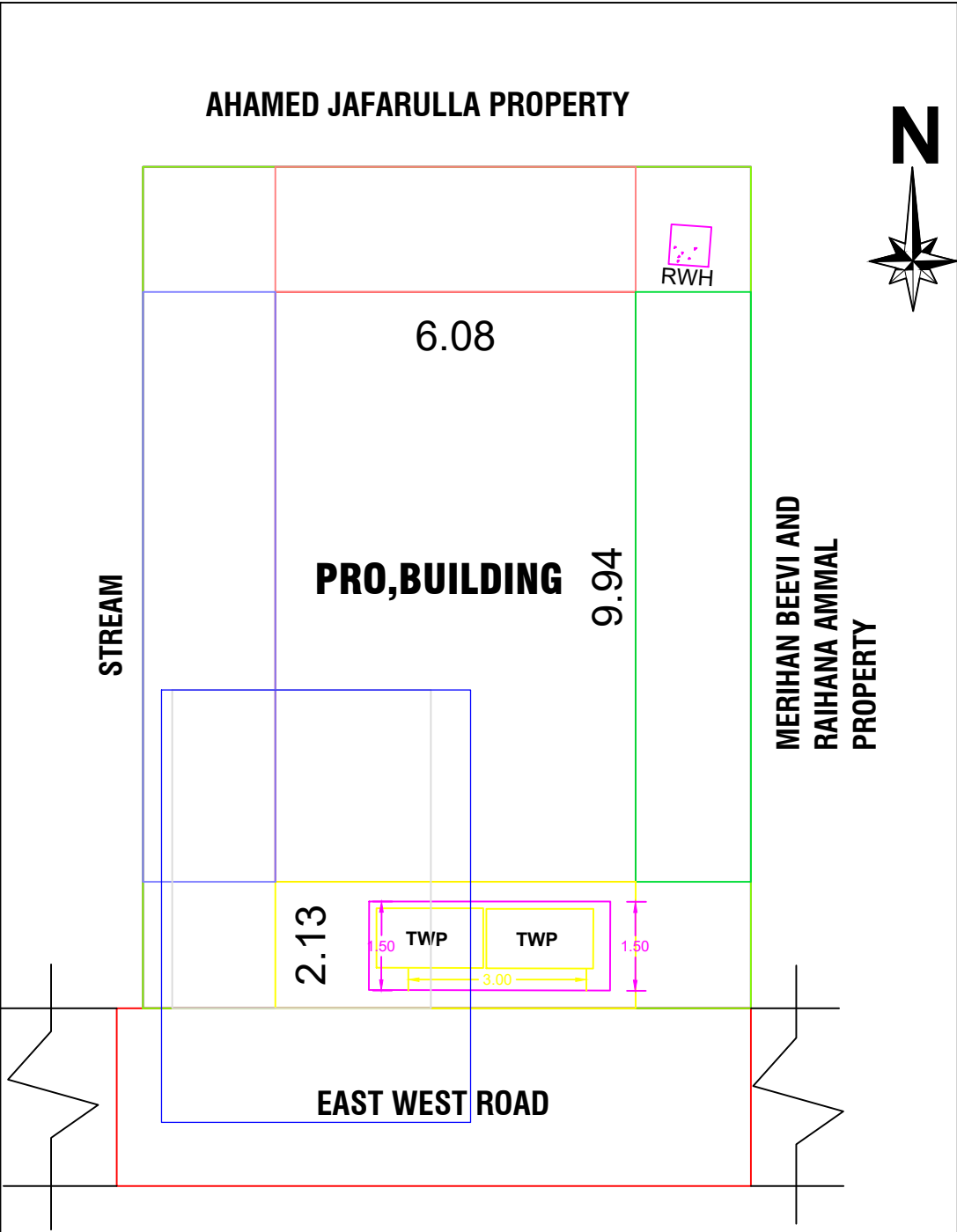
SITE PLAN
