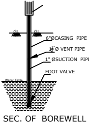
SEC. OF BOREWELL
