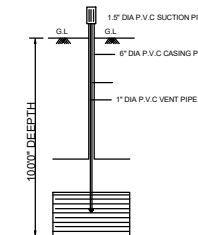
BORE WELL
